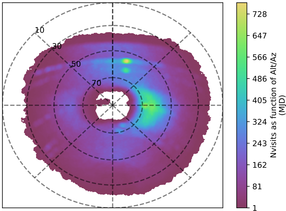
weather_cloudso4v3.4_10yrs u band: Nvisits as function of Alt/Az
