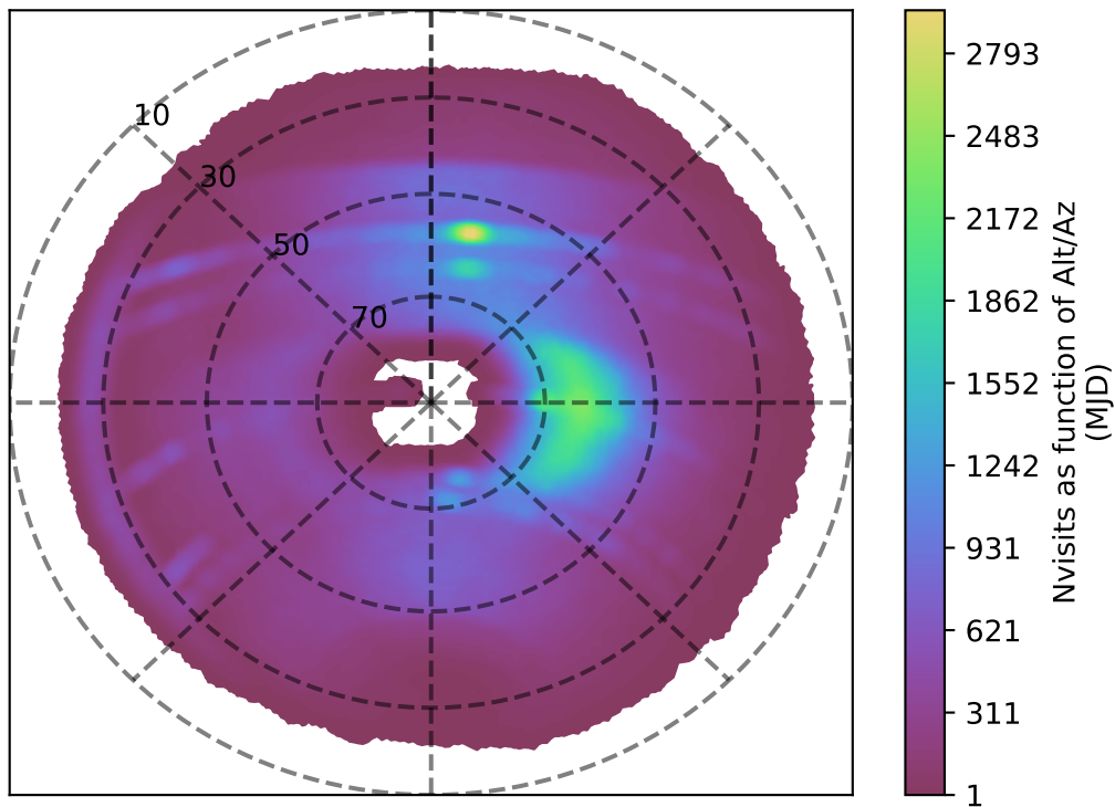
weather_cloudso4v3.4_10yrs r band: Nvisits as function of Alt/Az
