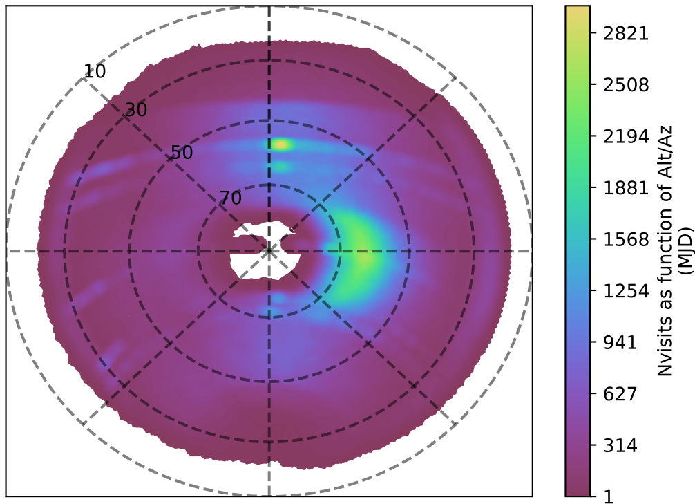
weather_cloudso4v3.4_10yrs i band: Nvisits as function of Alt/Az
