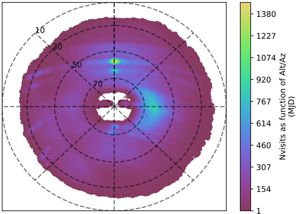
weather_cloudso4v3.4_10yrs g band: Nvisits as function of Alt/Az
