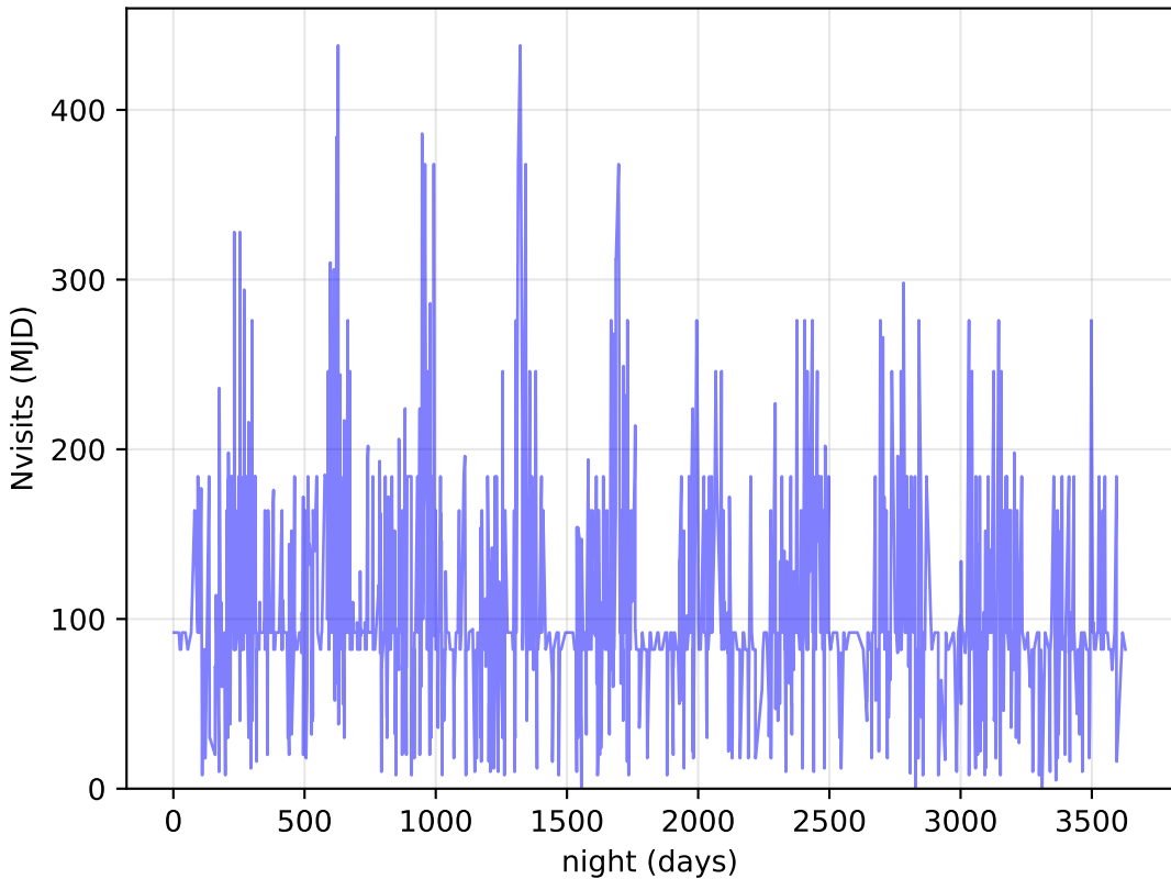
weather_cloudso4v3.4_10yrs DDF: Nvisits
