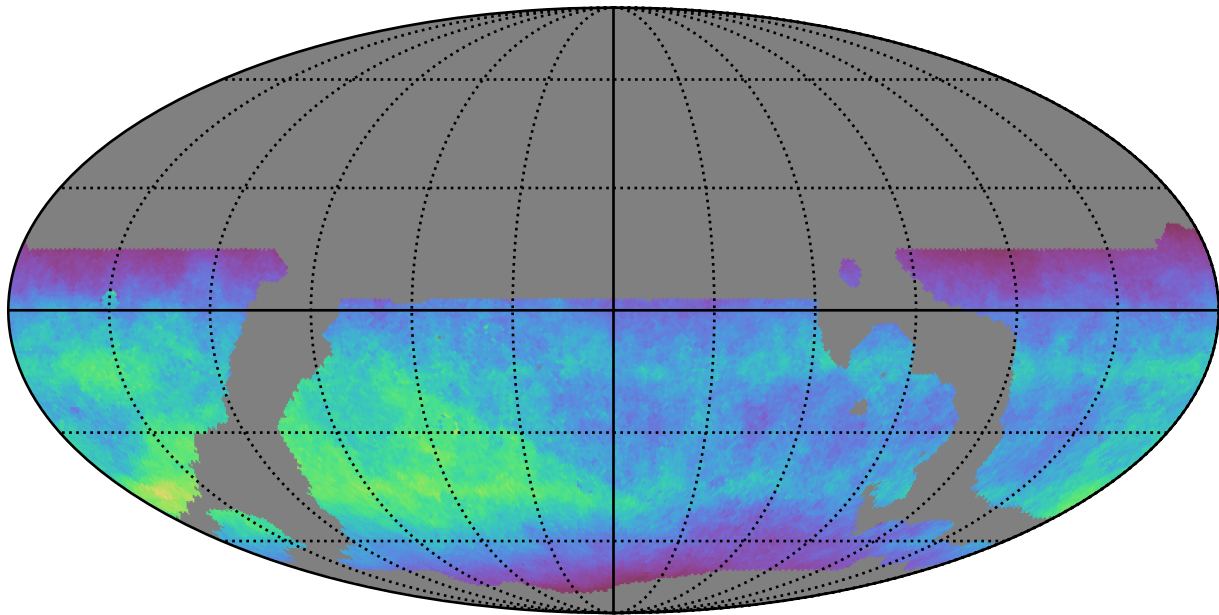
weather_cloudso4v3.4_10yrs WFD z band: Normalized Teff
