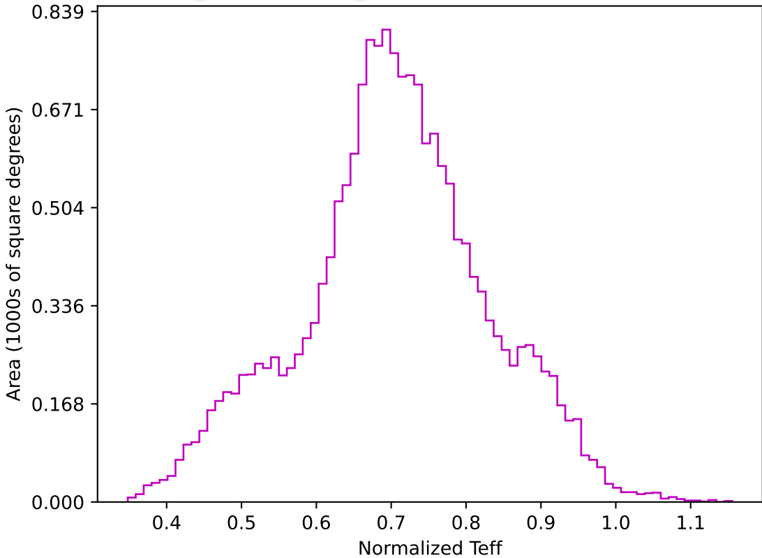
weather_cloudso4v3.4_10yrs WFD z band: Normalized Teff
