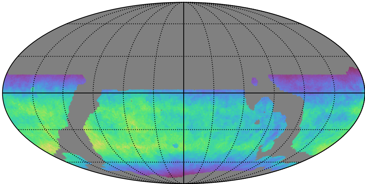
weather_cloudso4v3.4_10yrs WFD y band: Normalized Teff
