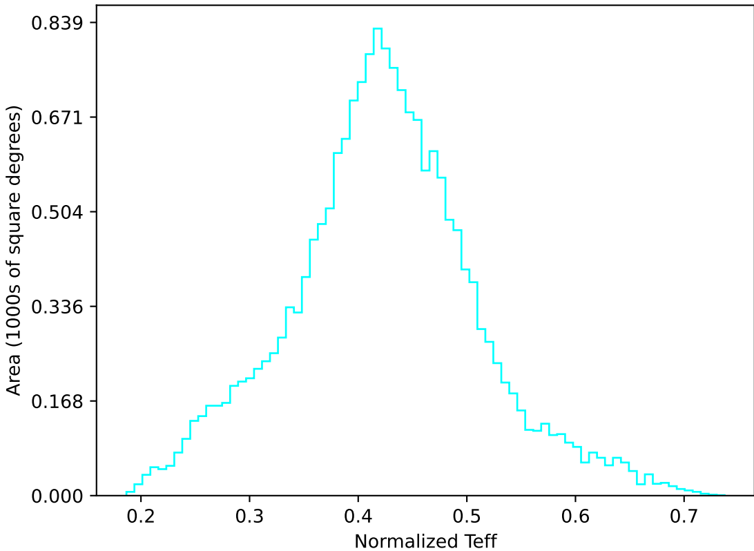
weather_cloudso4v3.4_10yrs WFD u band: Normalized Teff
