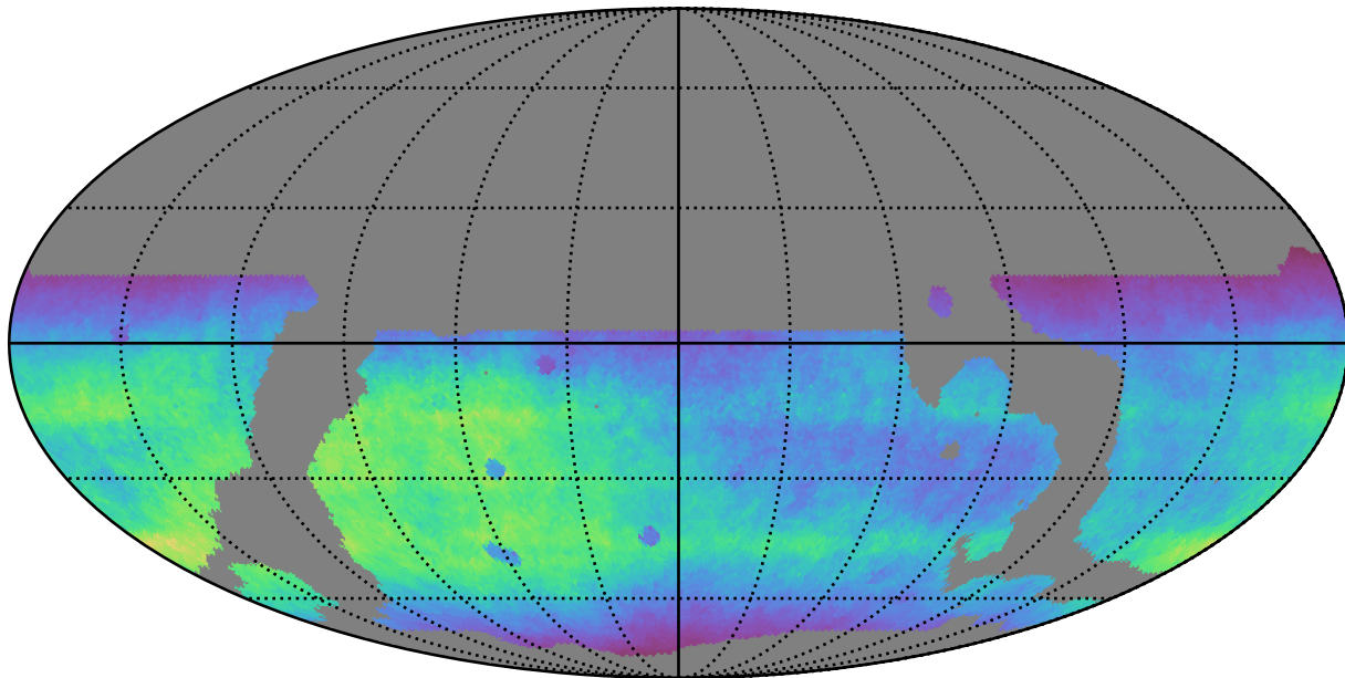
weather_cloudso4v3.4_10yrs WFD r band: Normalized Teff
