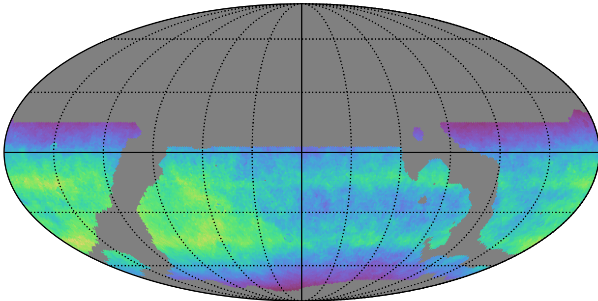
weather_cloudso4v3.4_10yrs WFD i band: Normalized Teff
