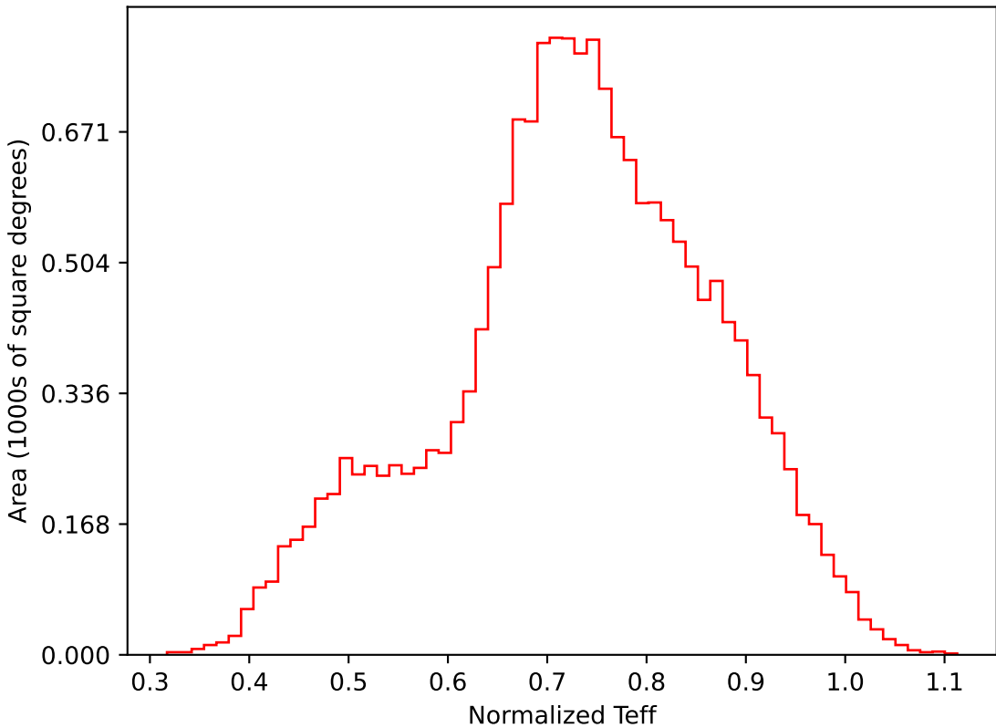
weather_cloudso4v3.4_10yrs WFD i band: Normalized Teff
