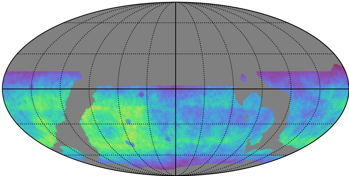
weather_cloudso4v3.4_10yrs WFD g band: Normalized Teff
