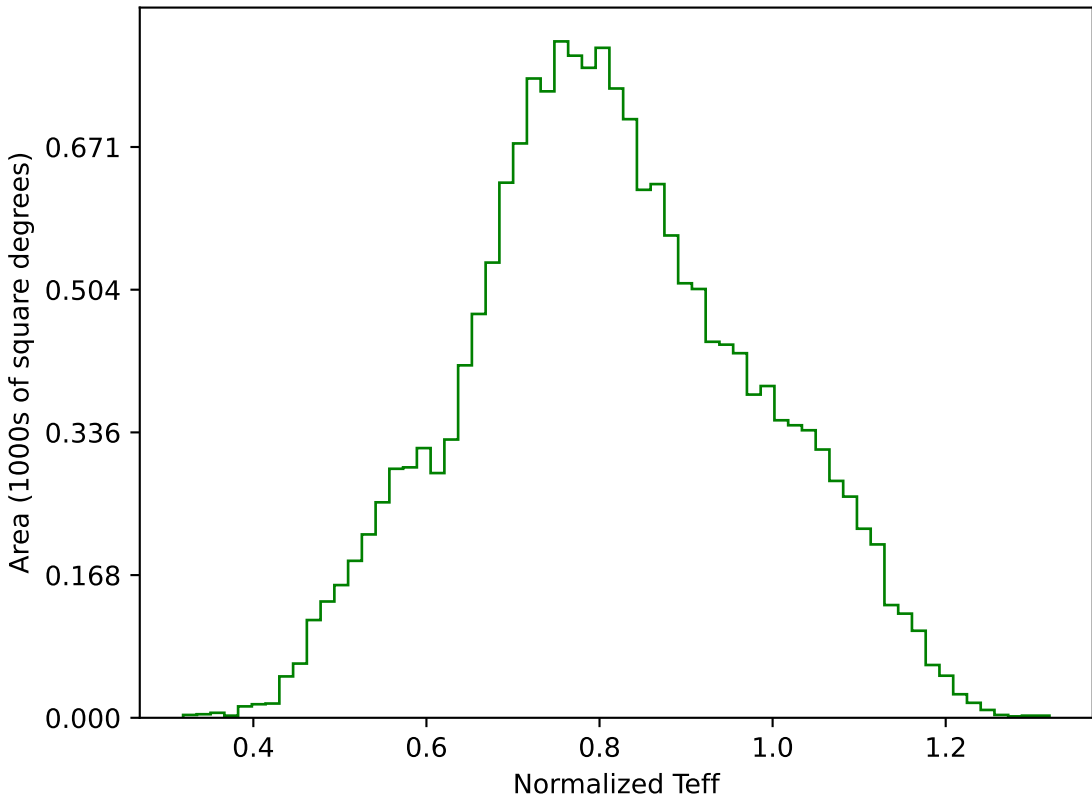
weather_cloudso4v3.4_10yrs WFD g band: Normalized Teff
