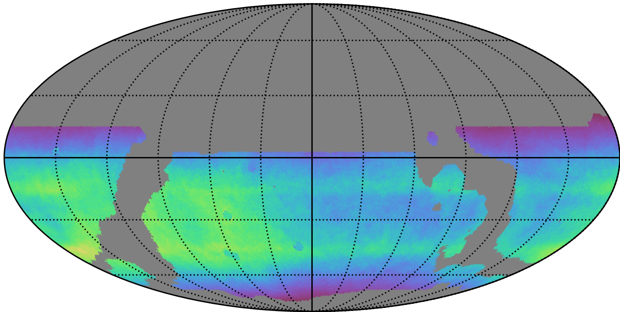
weather_cloudso4v3.4_10yrs WFD all bands: Normalized Teff
