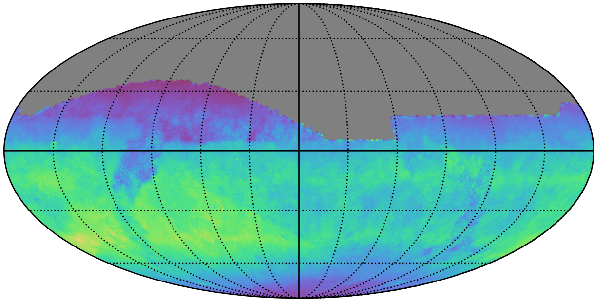
weather_cloudso4v3.4_10yrs All sky z band: Normalized Teff
