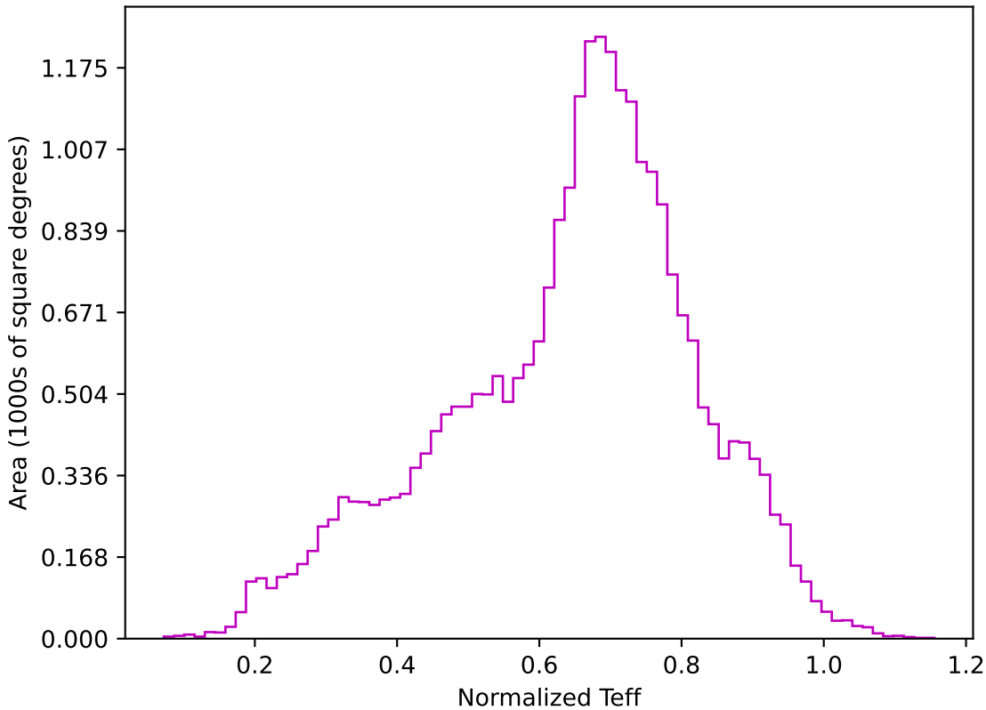
weather_cloudso4v3.4_10yrs All sky z band: Normalized Teff
