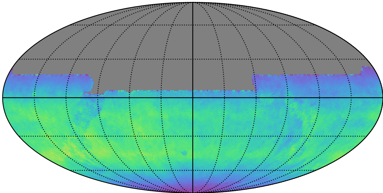
weather_cloudso4v3.4_10yrs All sky y band: Normalized Teff
