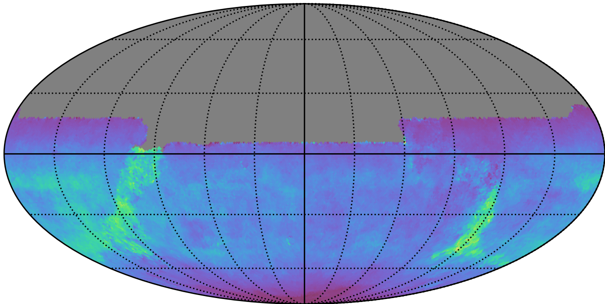
weather_cloudso4v3.4_10yrs All sky u band: Normalized Teff
