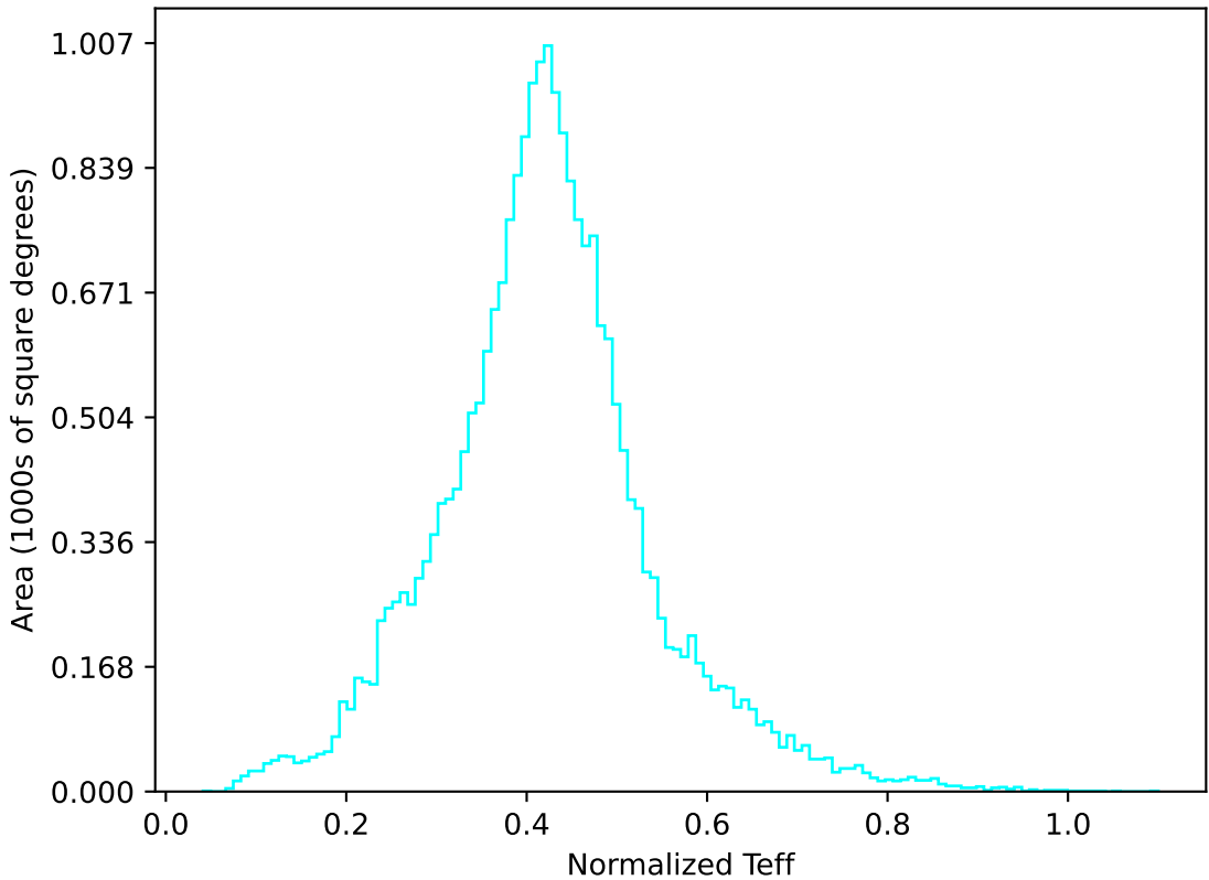
weather_cloudso4v3.4_10yrs All sky u band: Normalized Teff
