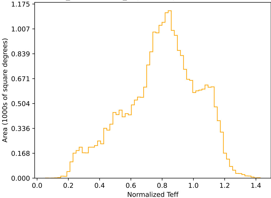
weather_cloudso4v3.4_10yrs All sky r band: Normalized Teff
