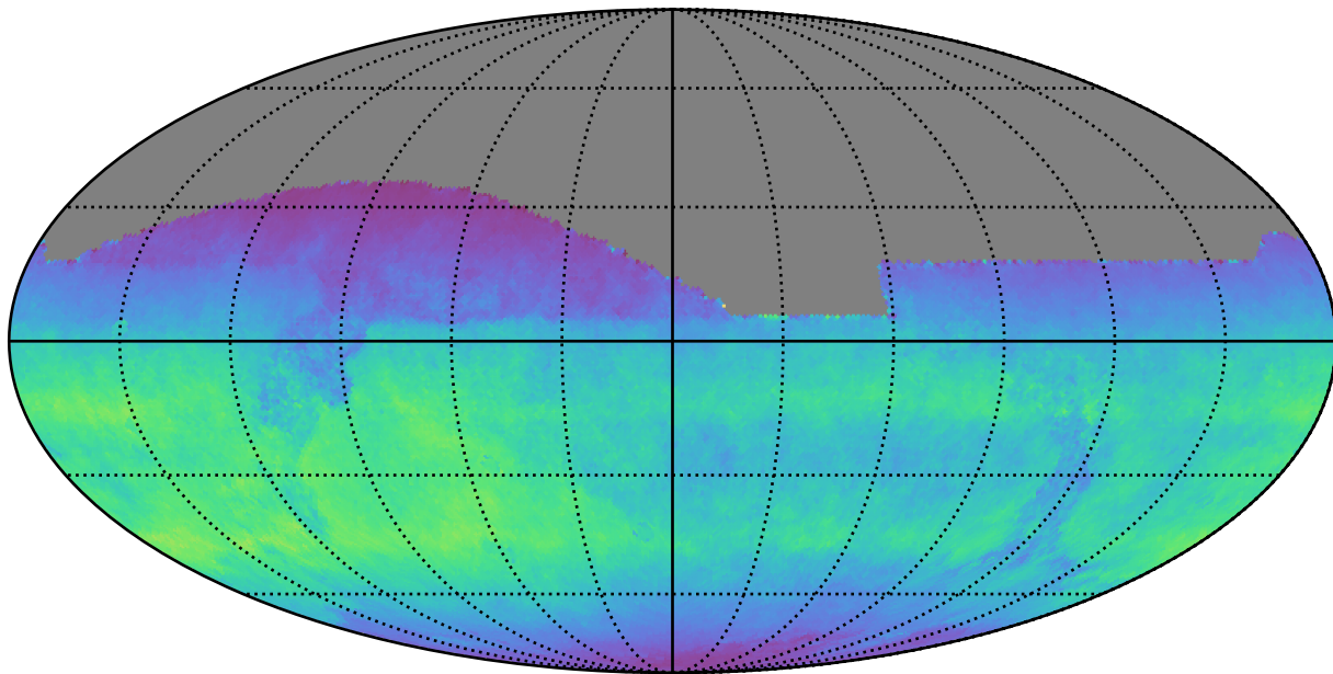
weather_cloudso4v3.4_10yrs All sky i band: Normalized Teff
