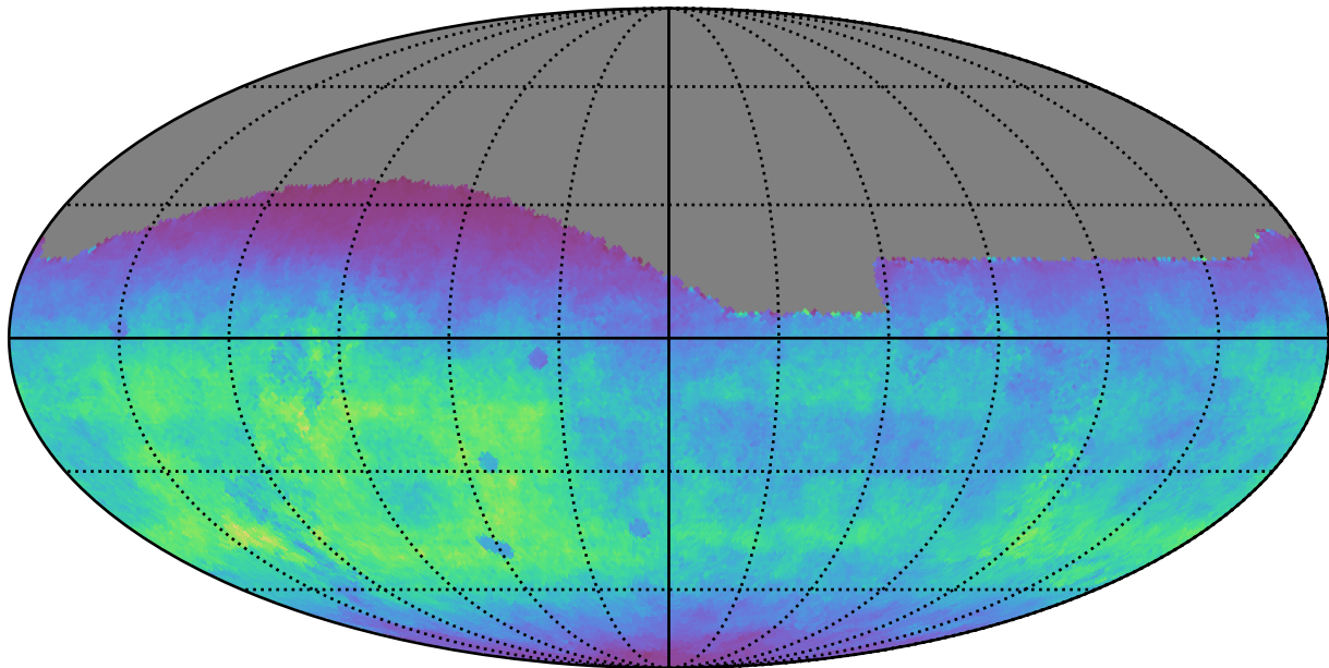
weather_cloudso4v3.4_10yrs All sky g band: Normalized Teff
