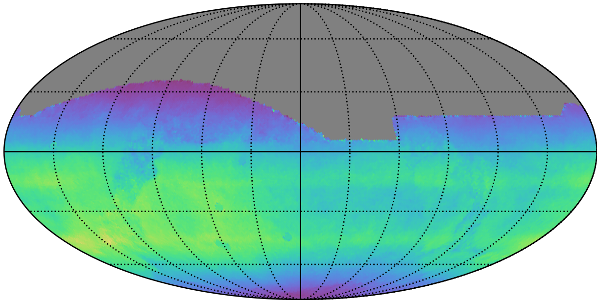
weather_cloudso4v3.4_10yrs All sky all bands: Normalized Teff
