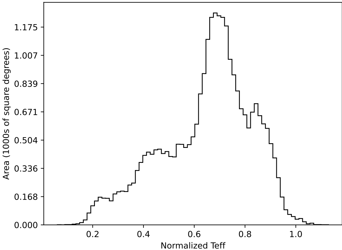
weather_cloudso4v3.4_10yrs All sky all bands: Normalized Teff
