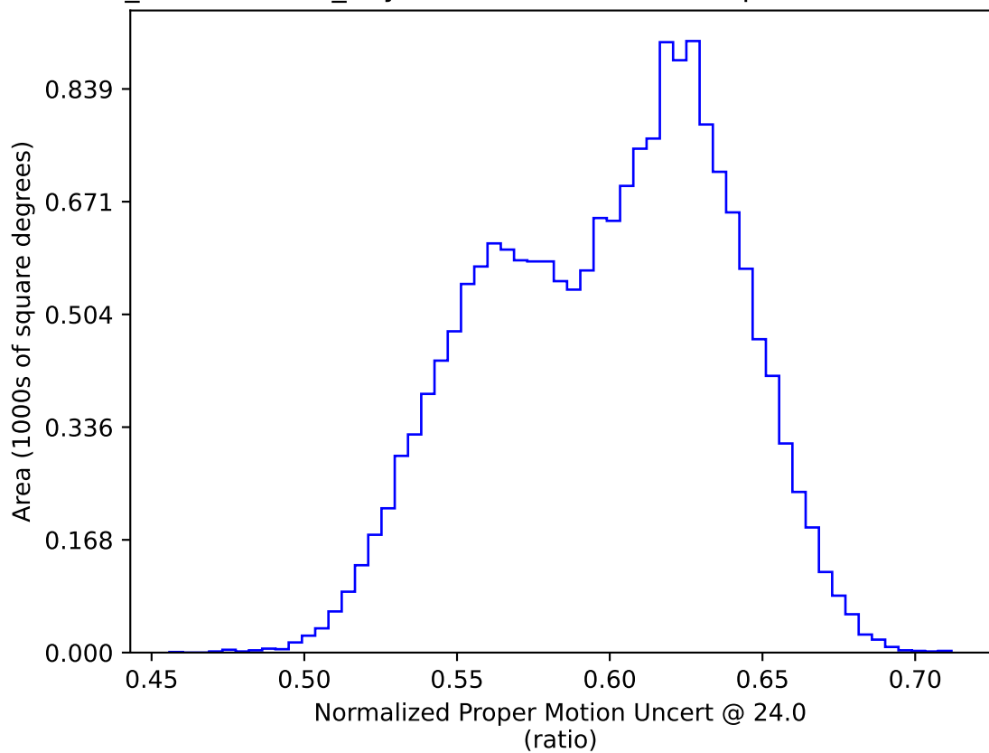
weather_cloudso4v3.4_10yrs WFD: Normalized Proper Motion Uncert @ 24.0
