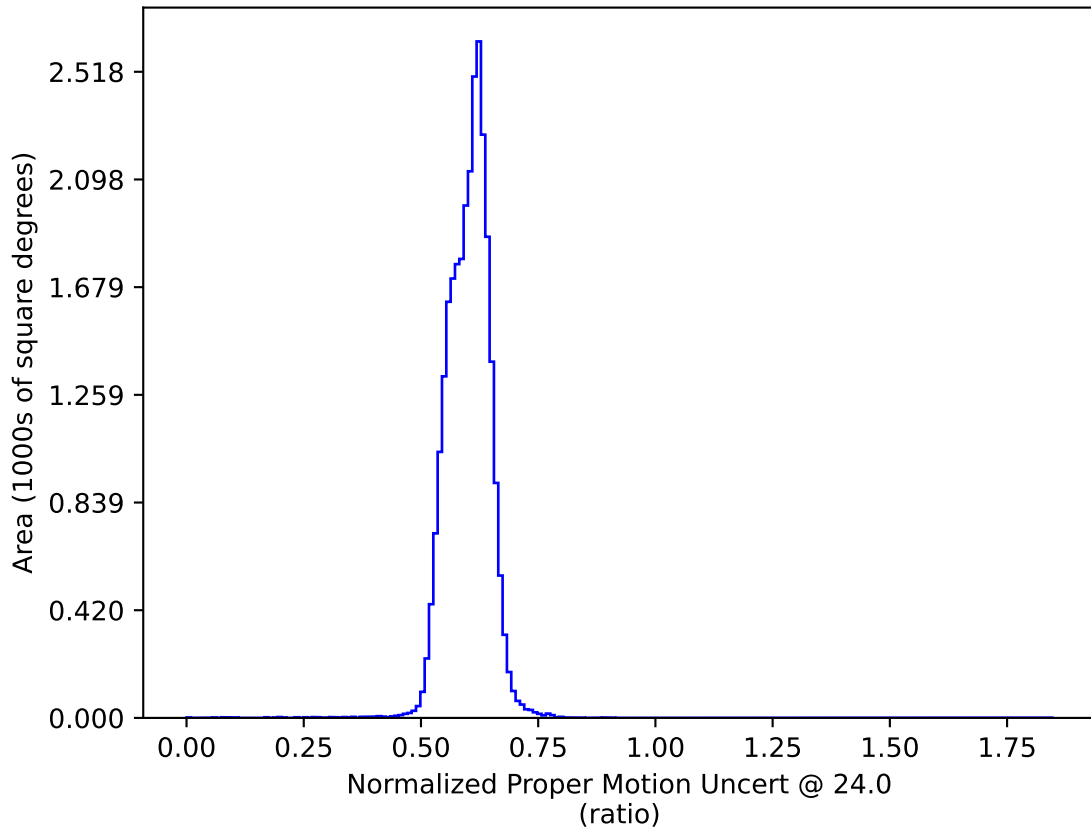
weather_cloudso4v3.4_10yrs All sky: Normalized Proper Motion Uncert @ 24.0
