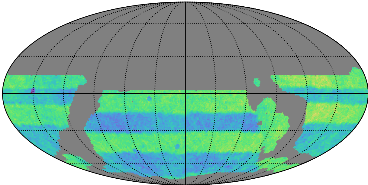
weather_cloudso4v3.4_10yrs WFD: Normalized Proper Motion Uncert @ 20.5
