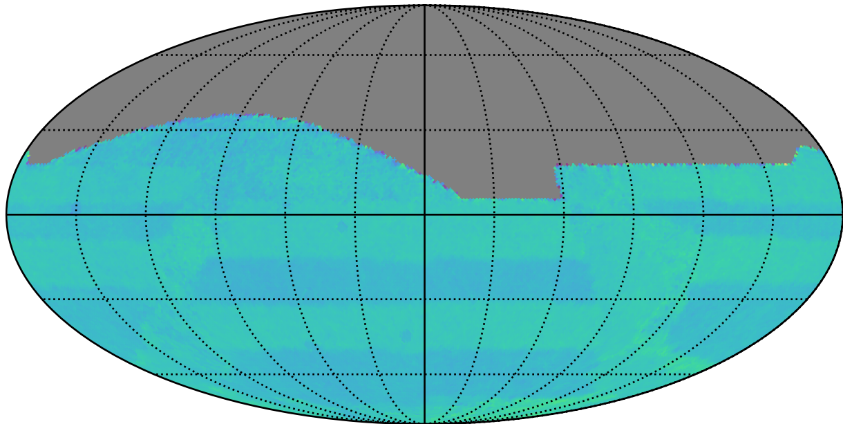
weather_cloudso4v3.4_10yrs All sky: Normalized Proper Motion Uncert @ 20.5
