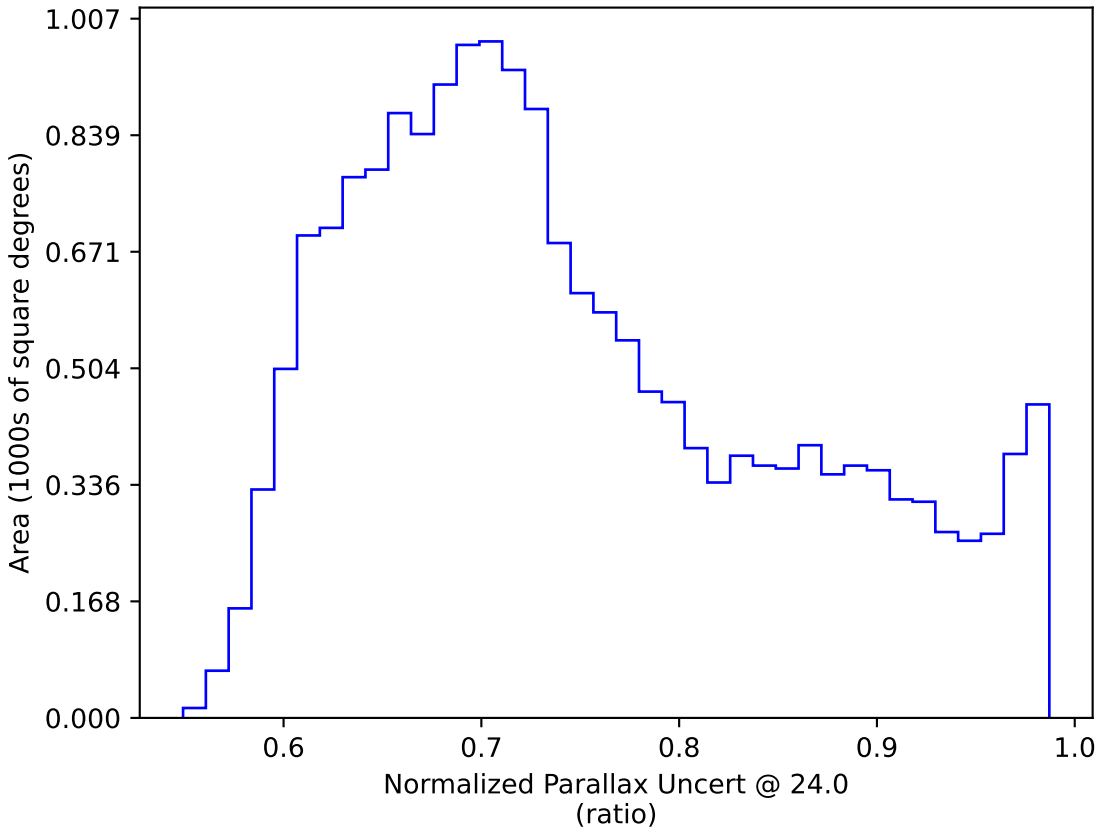
weather_cloudso4v3.4_10yrs WFD: Normalized Parallax Uncert @ 24.0
