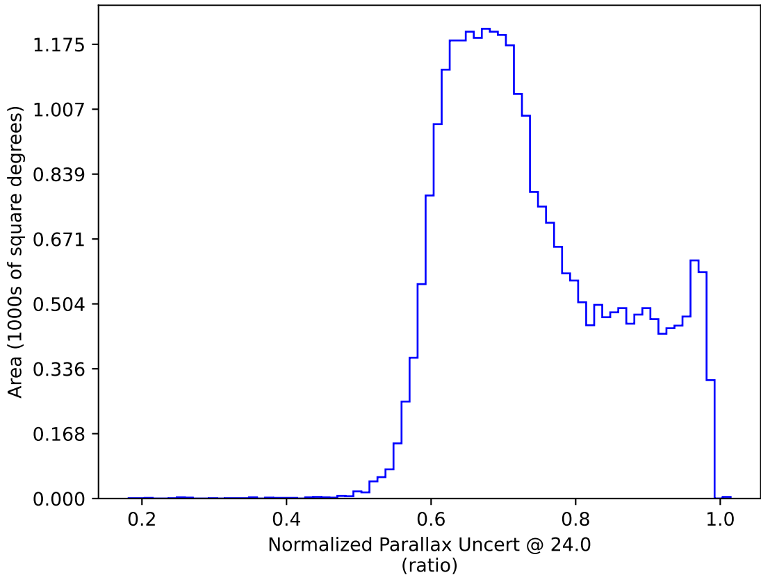
weather_cloudso4v3.4_10yrs All sky: Normalized Parallax Uncert @ 24.0
