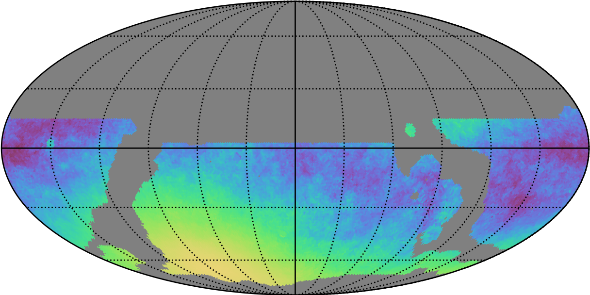
weather_cloudso4v3.4_10yrs WFD y band only: Normalized Parallax Uncert @ 21.3
