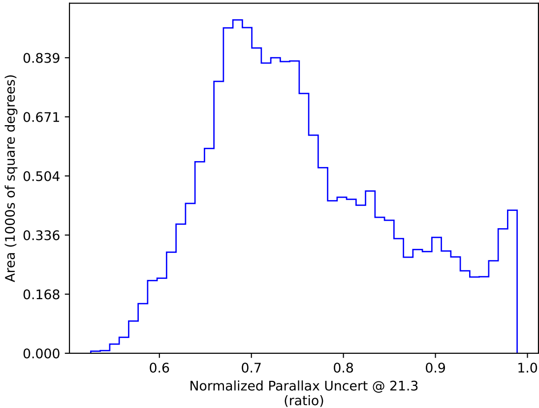
weather_cloudso4v3.4_10yrs WFD y band only: Normalized Parallax Uncert @ 21.3
