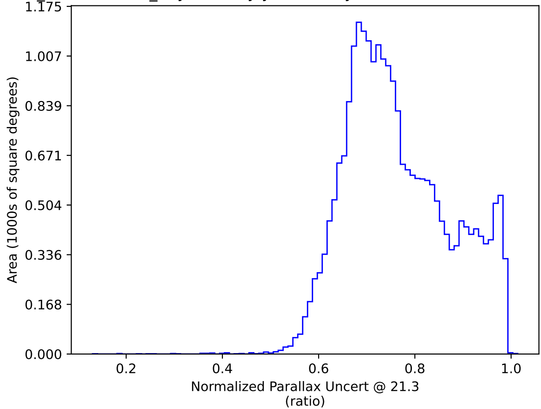
weather_cloudso4v3.4_10yrs All sky y band only: Normalized Parallax Uncert @ 21.3
