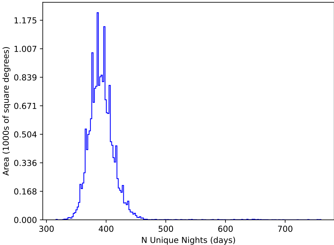
weather_cloudso4v3.4_10yrs WFD all bands: N Unique Nights
