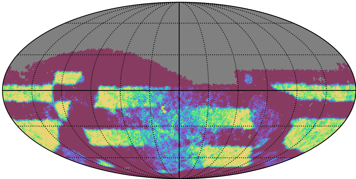
weather_cloudso4v3.4_10yrs Yr 3-4 z band: NVisits
