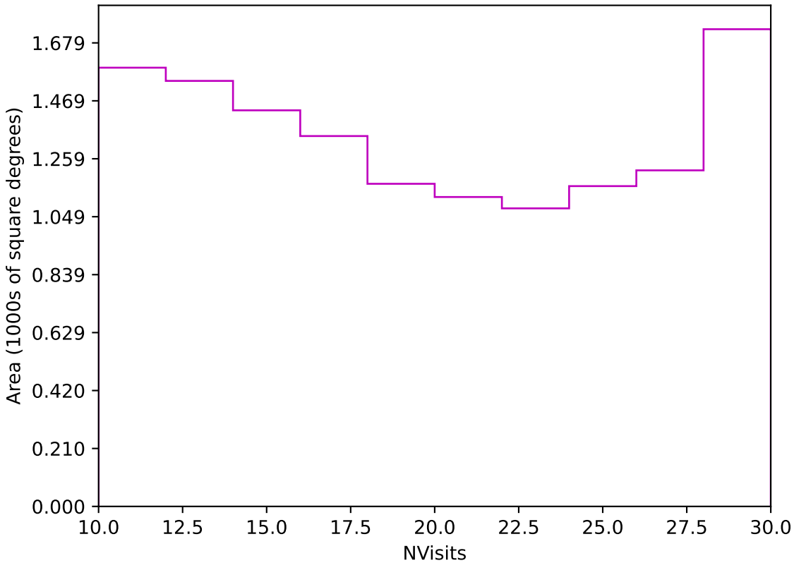
weather_cloudso4v3.4_10yrs Yr 3-4 z band: NVisits
