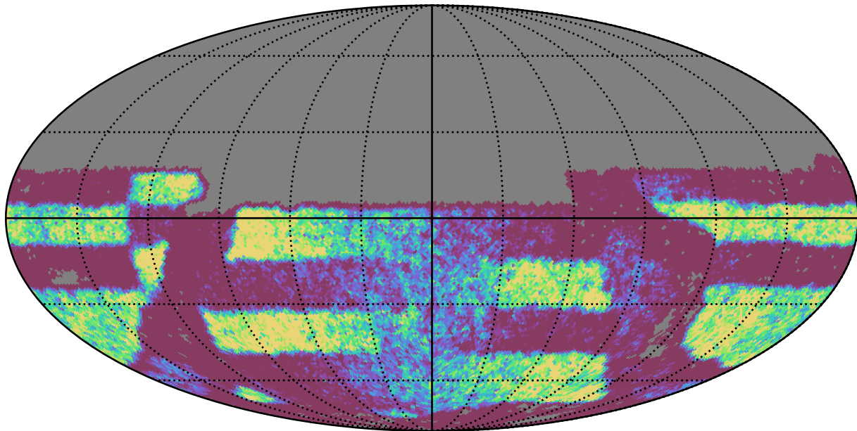
weather_cloudso4v3.4_10yrs Yr 3-4 y band: NVisits
