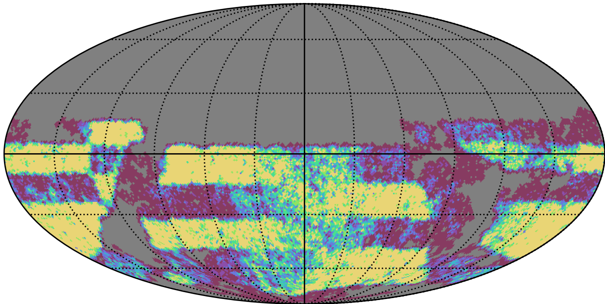
weather_cloudso4v3.4_10yrs Yr 3-4 u band: NVisits
