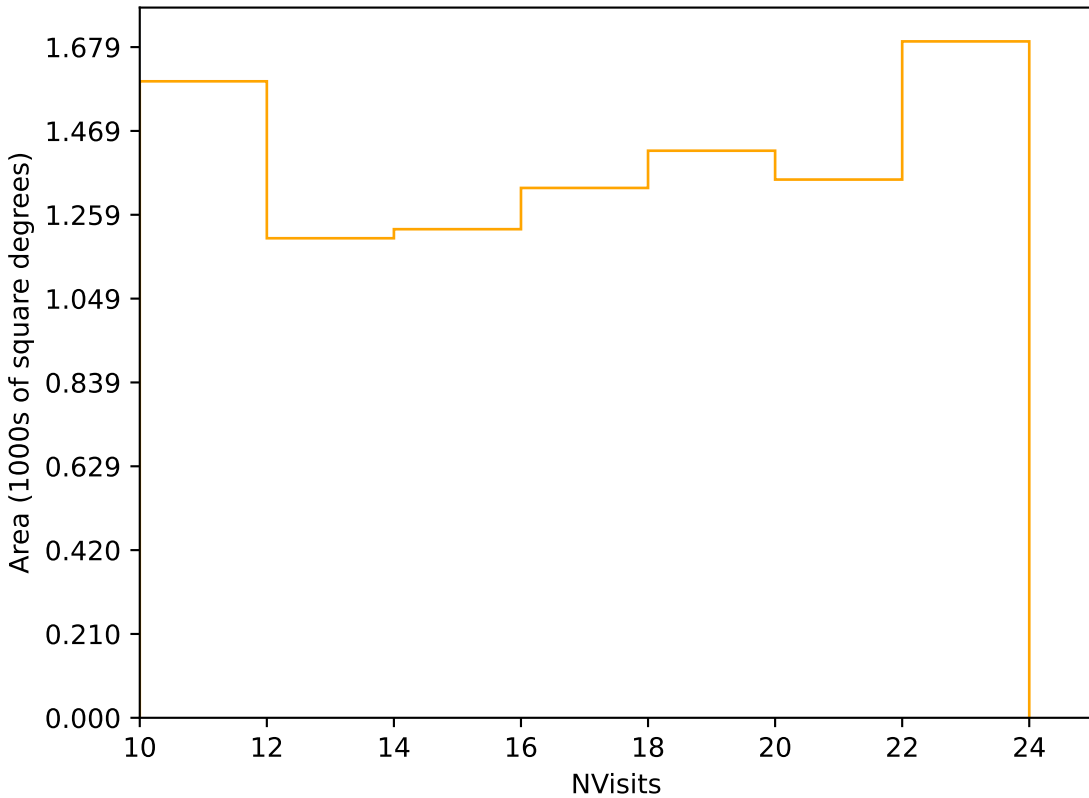
weather_cloudso4v3.4_10yrs Yr 3-4 r band: NVisits
