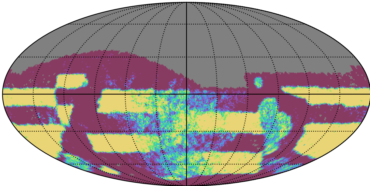
weather_cloudso4v3.4_10yrs Yr 3-4 i band: NVisits
