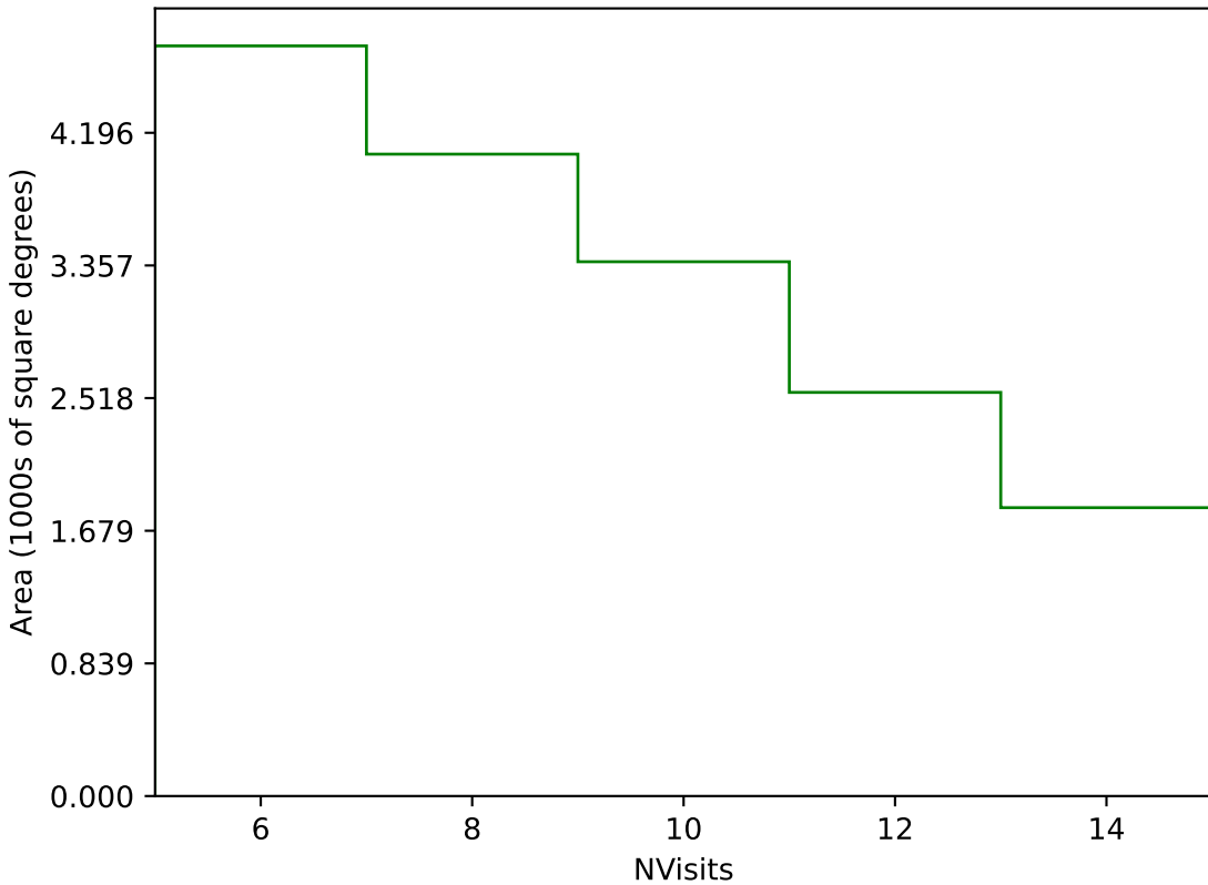
weather_cloudso4v3.4_10yrs Yr 3-4 g band: NVisits
