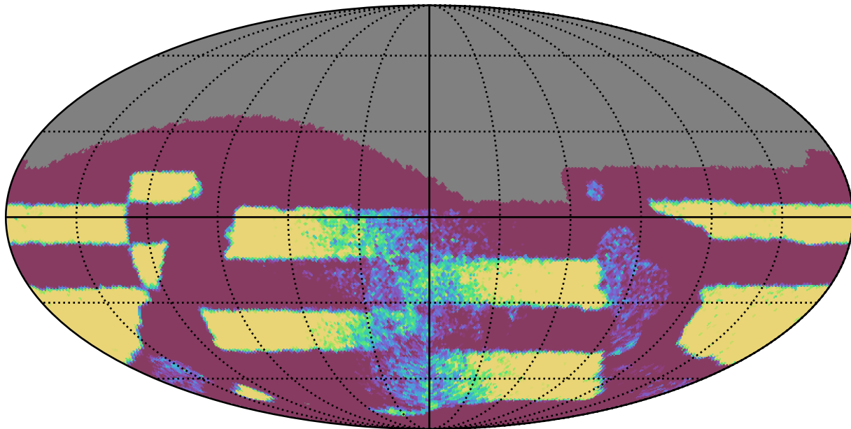
weather_cloudso4v3.4_10yrs Yr 3-4 all bands: NVisits
