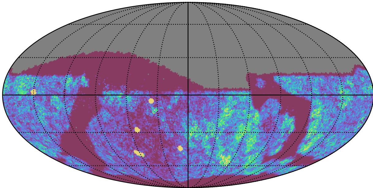
weather_cloudso4v3.4_10yrs Yr 1 z band: NVisits
