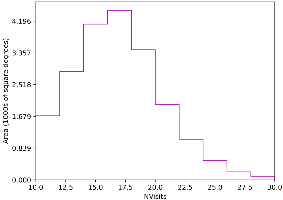
weather_cloudso4v3.4_10yrs Yr 1 z band: NVisits
