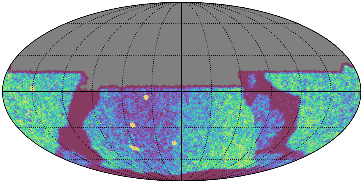
weather_cloudso4v3.4_10yrs Yr 1 y band: NVisits
