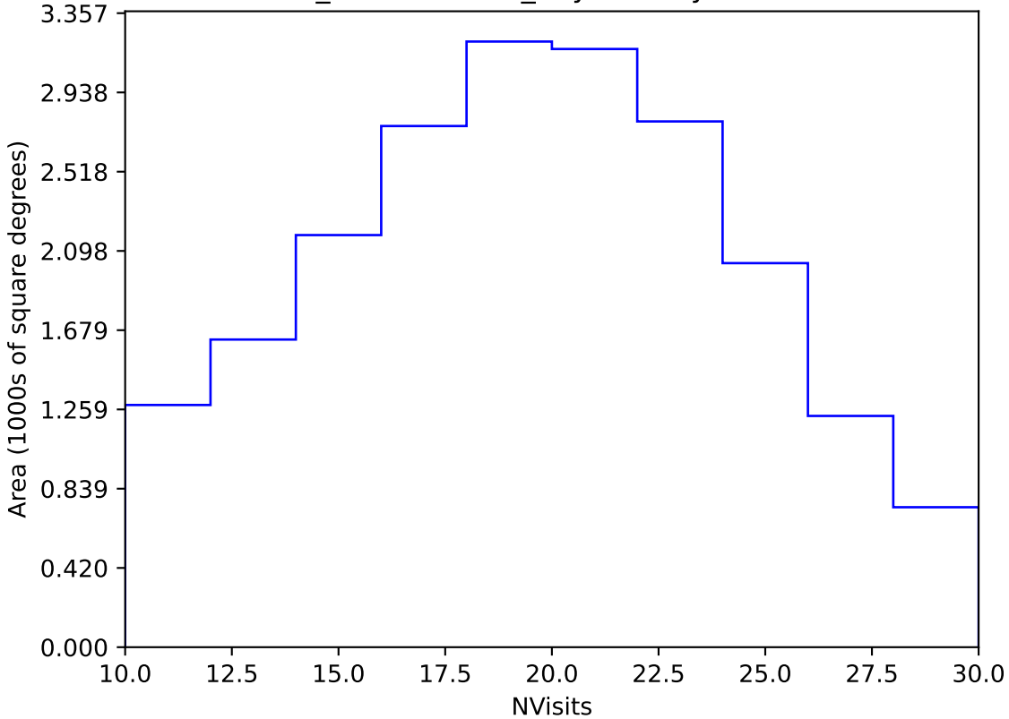
weather_cloudso4v3.4_10yrs Yr 1 y band: NVisits
