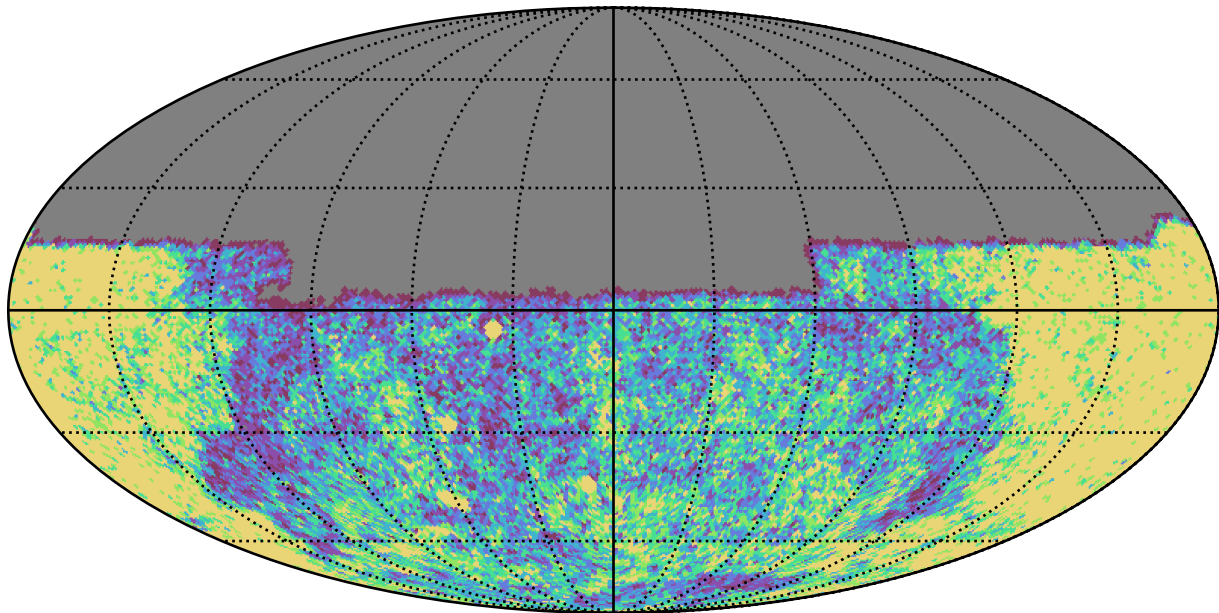
weather_cloudso4v3.4_10yrs Yr 1 u band: NVisits
