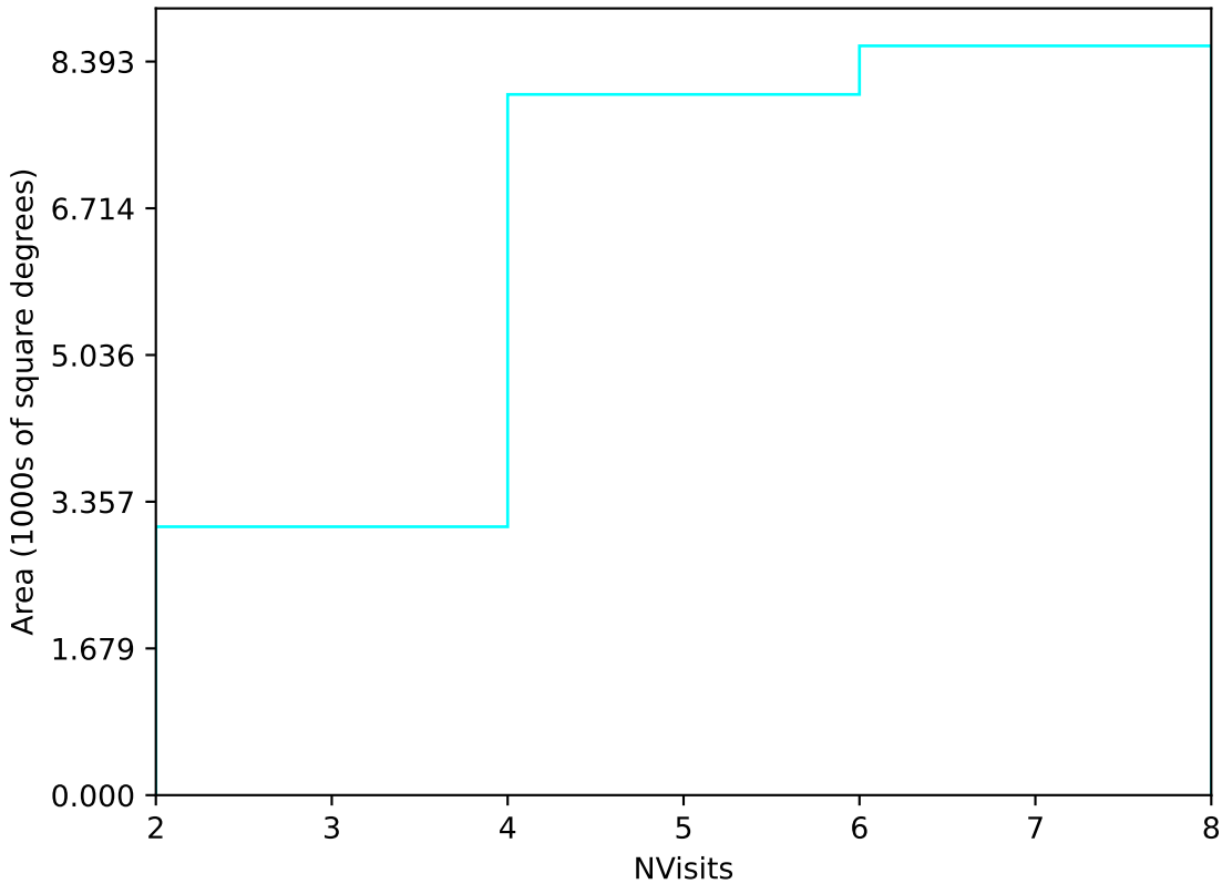
weather_cloudso4v3.4_10yrs Yr 1 u band: NVisits
