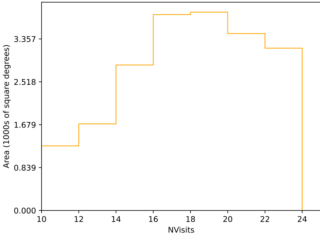
weather_cloudso4v3.4_10yrs Yr 1 r band: NVisits
